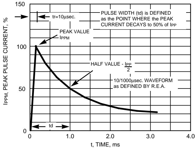
FIG. 3 - PULSE WAVEFORM
